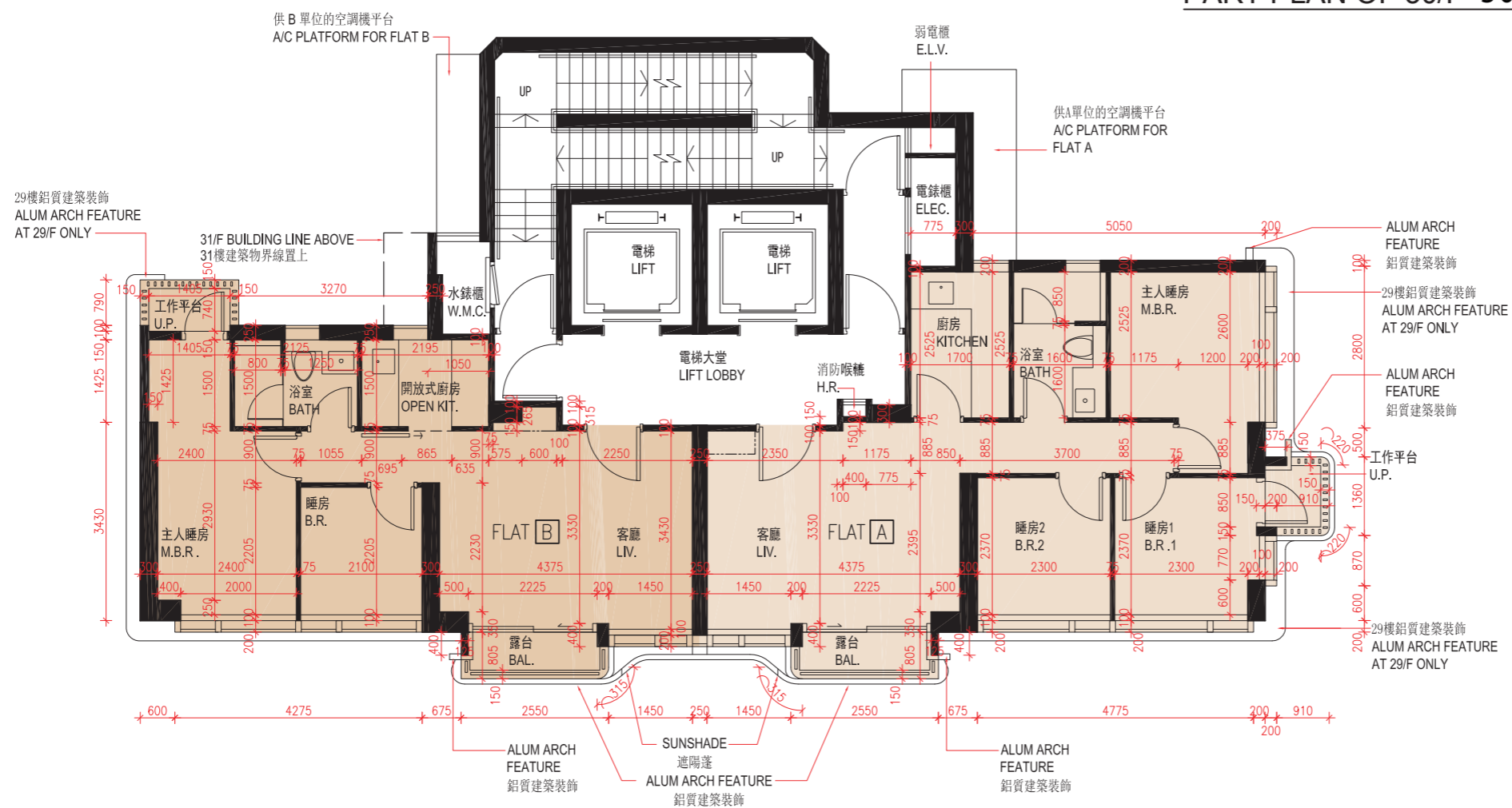
PART PLAN OF 30/F 30樓部分平面圖
