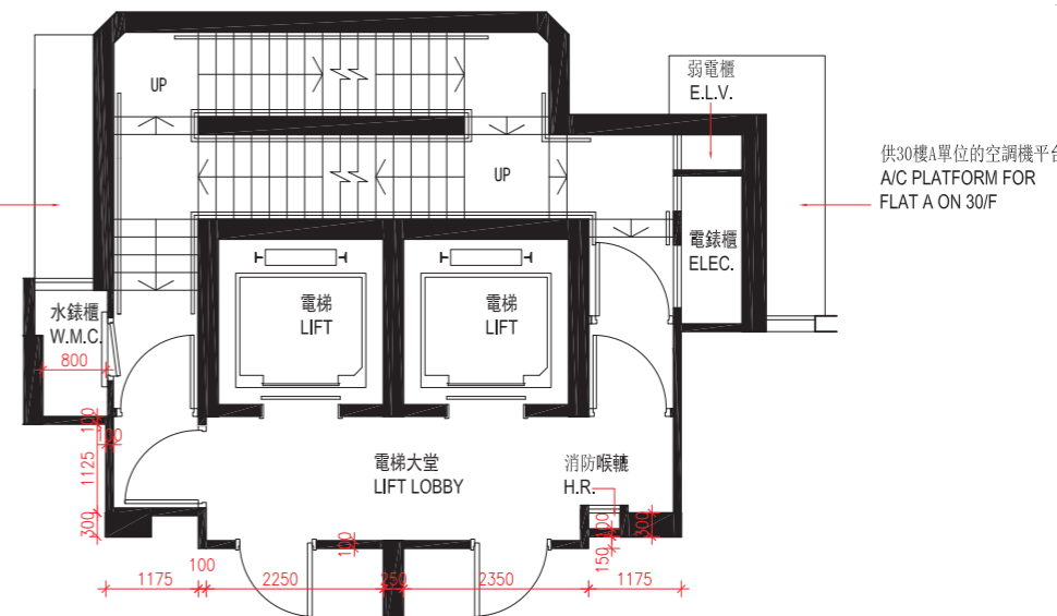
PART PLAN OF 30/F 30樓部分平面圖
